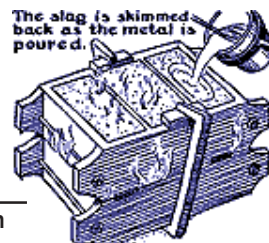
The slag is skimmed back as the metal is poured. The cope and drag are clamped together.
